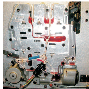
700-R4 Assembled
