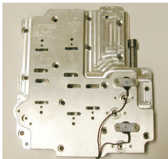
2004R Billet Valve Body
