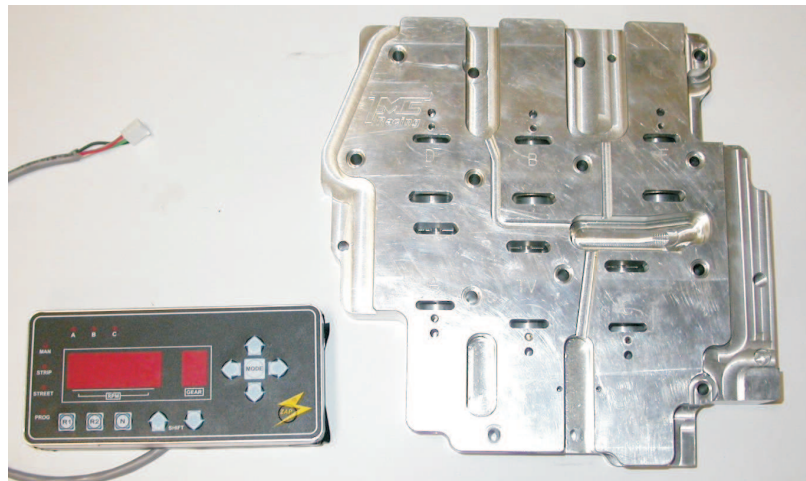
700-R4 Billet Valve Body and Controller
